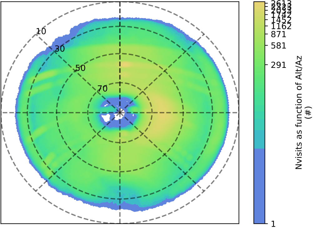
too_elab_2yr_r64_d3_ugrizy_v3.4_10yrs i: Nvisits as function of Alt/Az
