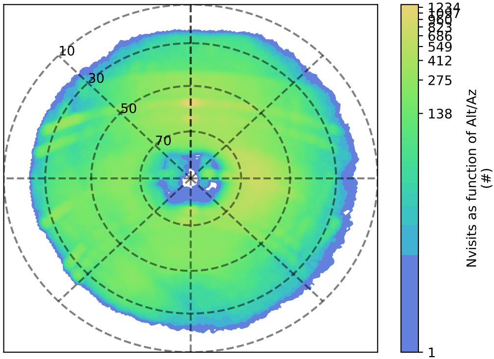
too_elab_2yr_r64_d3_ugrizy_v3.4_10yrs g: Nvisits as function of Alt/Az
