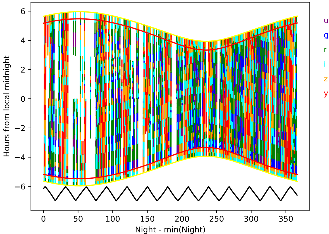
too_elab_2yr_r64_d3_ugrizy_v3.4_10yrs year 9-10: Hourglass
