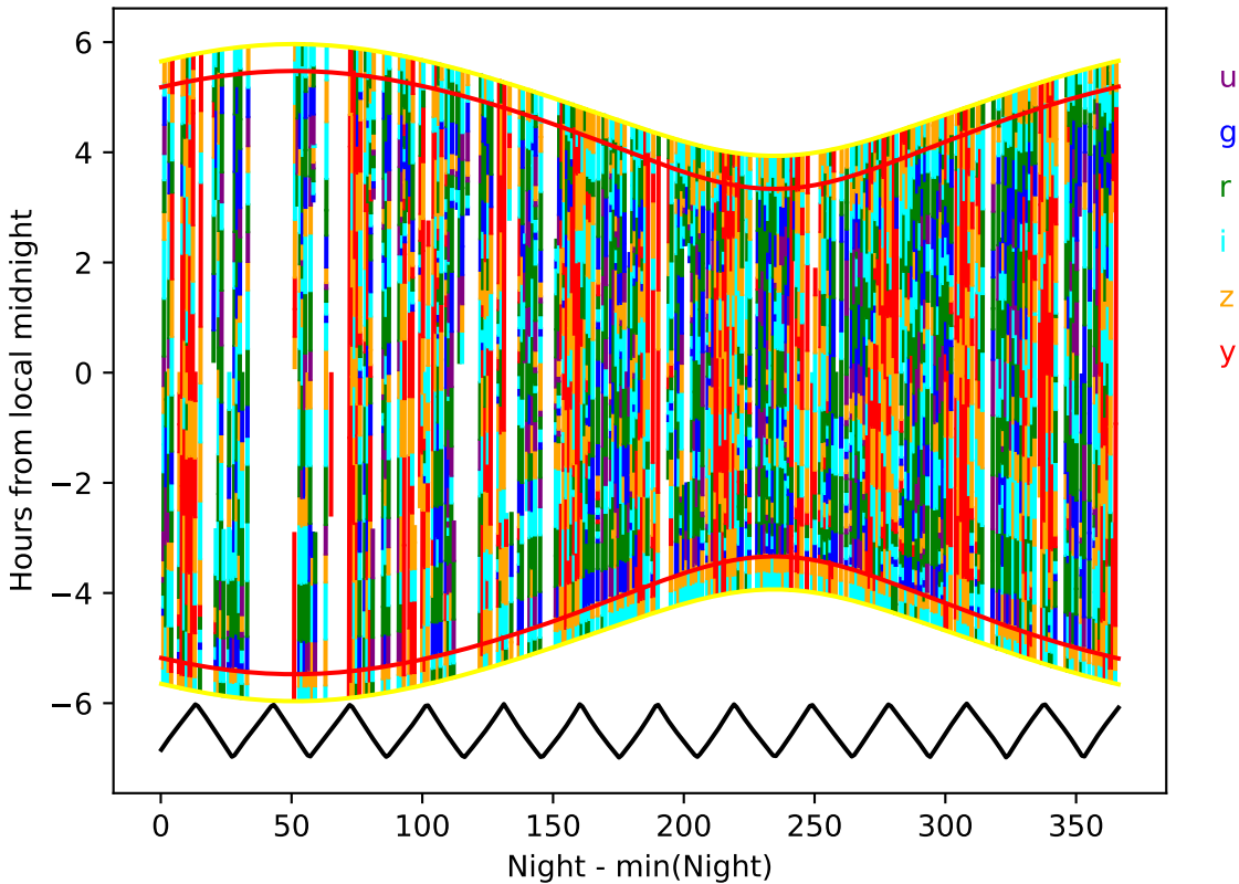
too_elab_2yr_r64_d3_ugrizy_v3.4_10yrs year 8-9: Hourglass
