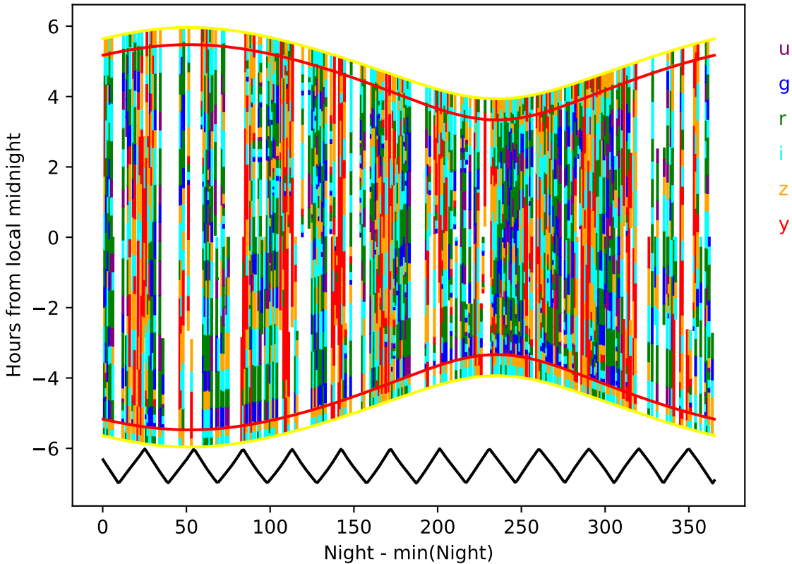
too_elab_2yr_r64_d3_ugrizy_v3.4_10yrs year 7-8: Hourglass
