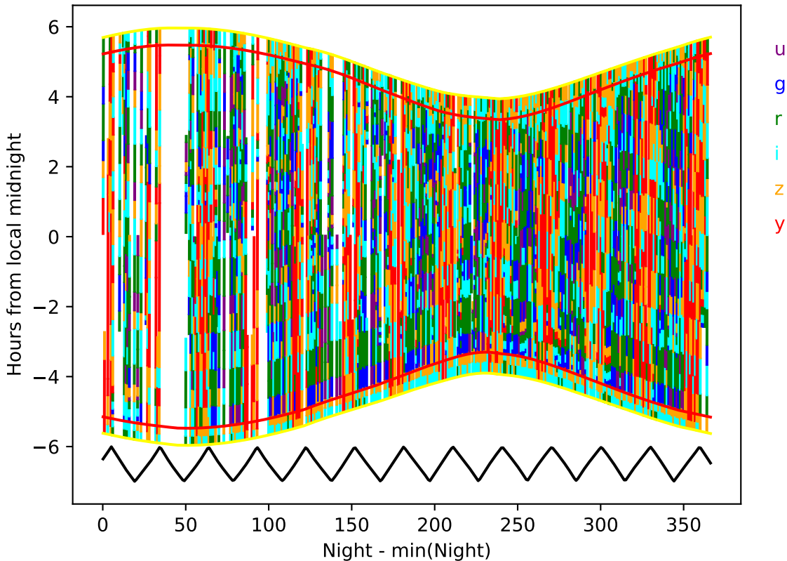
too_elab_2yr_r64_d3_ugrizy_v3.4_10yrs year 6-7: Hourglass
