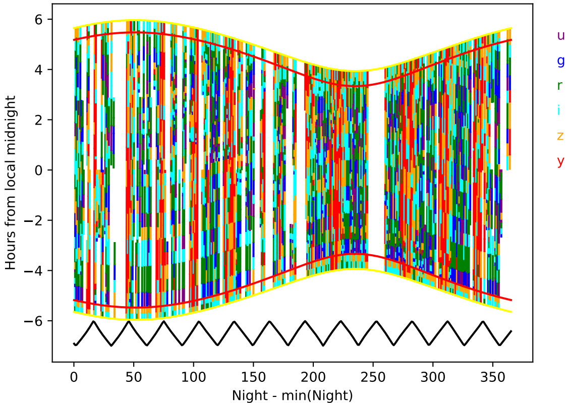
too_elab_2yr_r64_d3_ugrizy_v3.4_10yrs year 5-6: Hourglass
