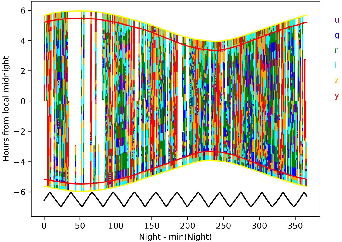
too_elab_2yr_r64_d3_ugrizy_v3.4_10yrs year 3-4: Hourglass
