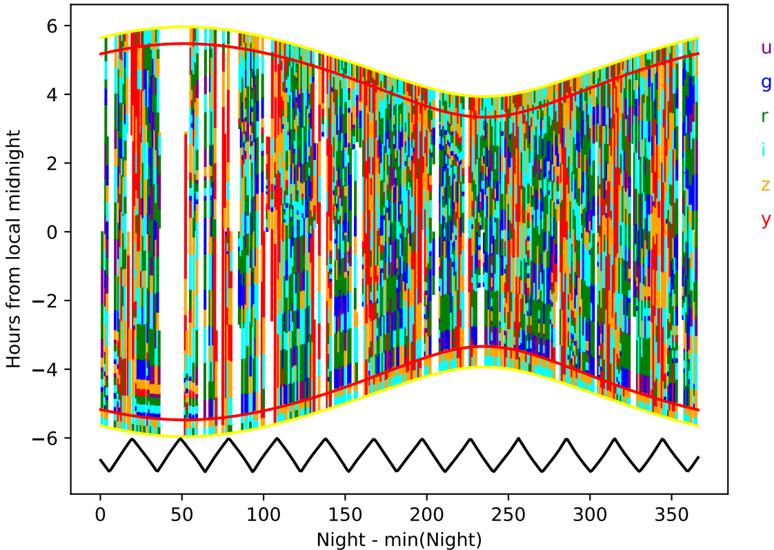
too_elab_2yr_r64_d3_ugrizy_v3.4_10yrs year 2-3: Hourglass
