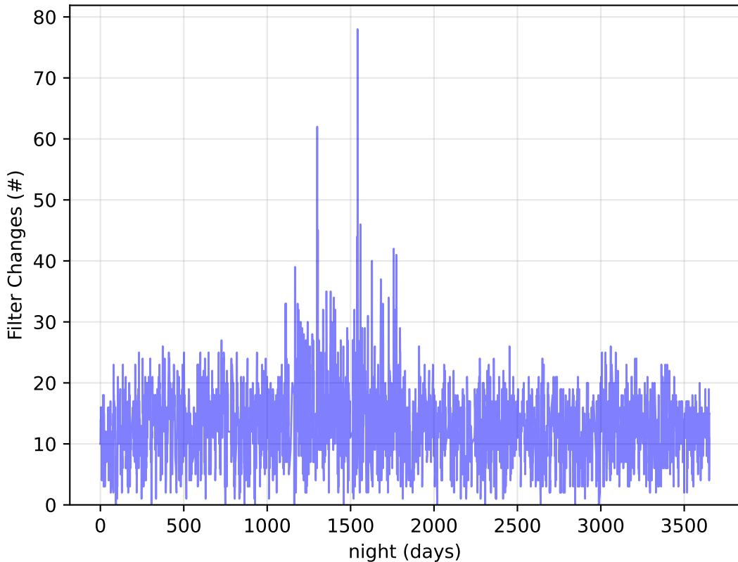
too_elab_2yr_r64_d3_ugrizy_v3.4_10yrs : Filter Changes
