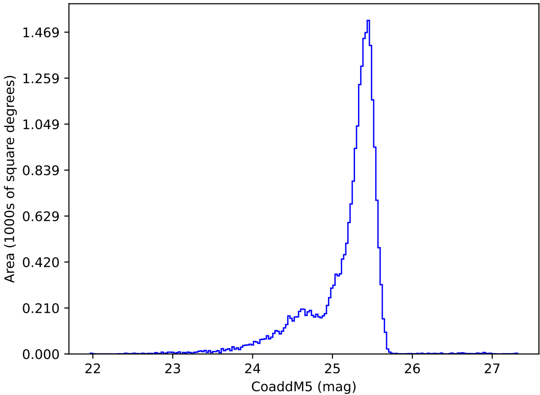
too_elab_2yr_r64_d3_ugrizy_v3.4_10yrs u: CoaddM5
