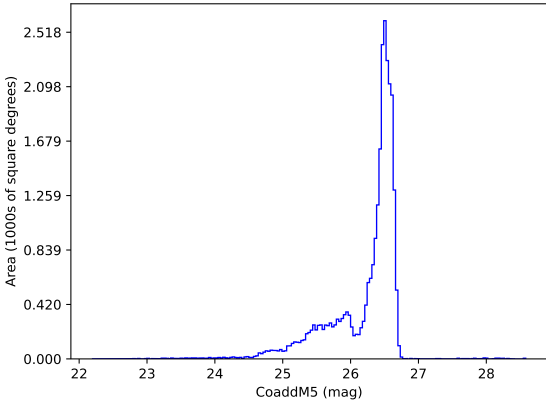
too_elab_2yr_r64_d3_ugrizy_v3.4_10yrs i: CoaddM5
