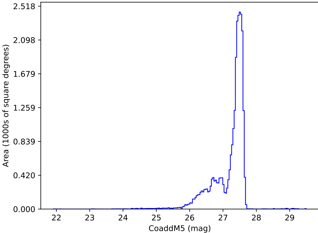
too_elab_2yr_r64_d3_ugrizy_v3.4_10yrs : CoaddM5
