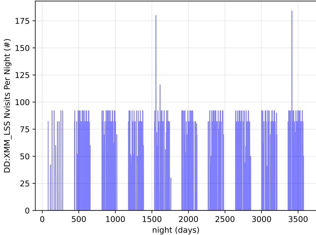
too_elab_2yr_r64_d3_ugrizy_v3.4_10yrs all bands: DD:XMM_LSS Nvisits Per Night
