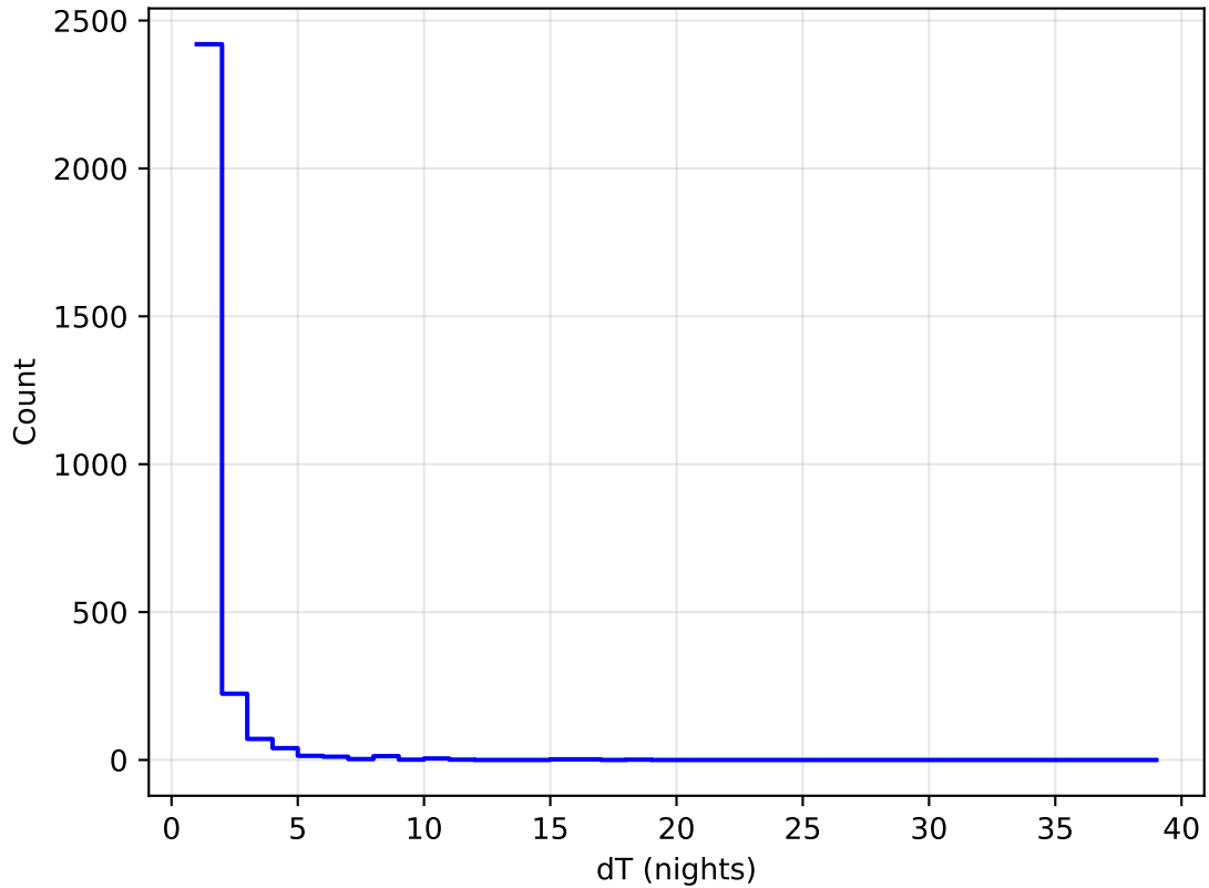
too_elab_2yr_r64_d3_ugrizy_v3.4_10yrs all bands: DD:WFD Delta Nights Histogram
