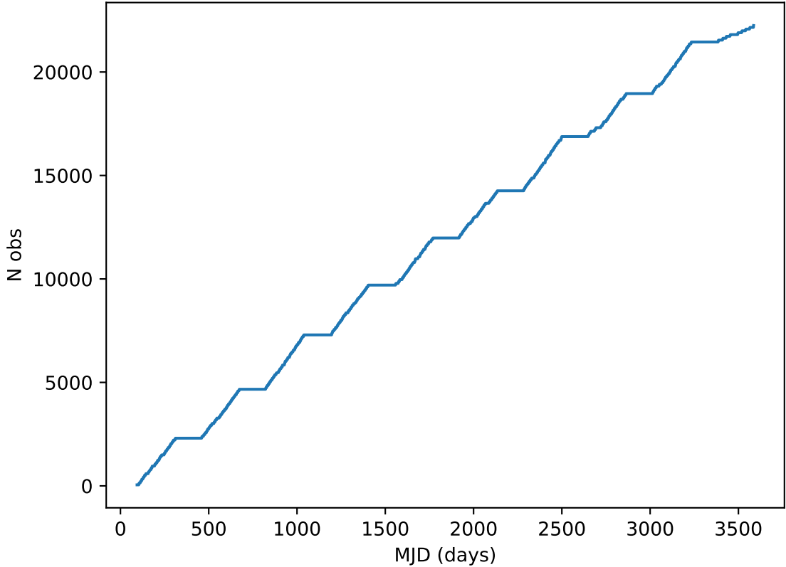
too_elab_2yr_r64_d3_ugrizy_v3.4_10yrs all bands: DD:ECDFS Cumulative NVisits
