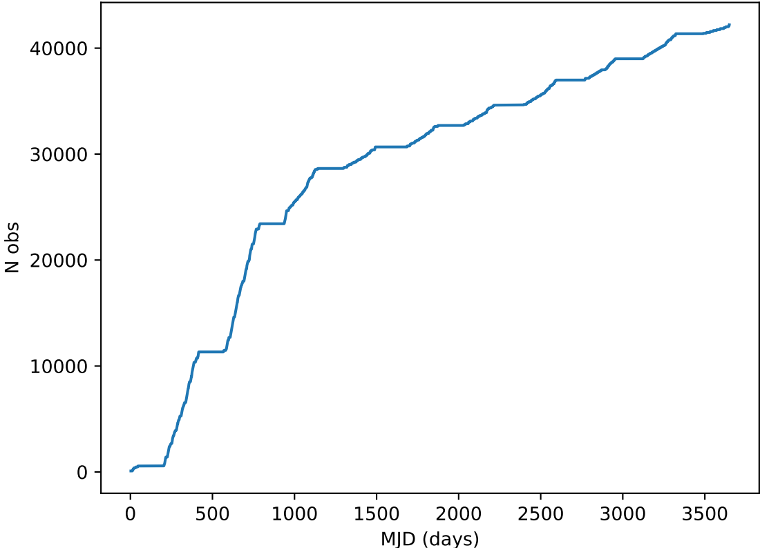
too_elab_2yr_r64_d3_ugrizy_v3.4_10yrs all bands: DD: COSMOS Cumulative NVisits
