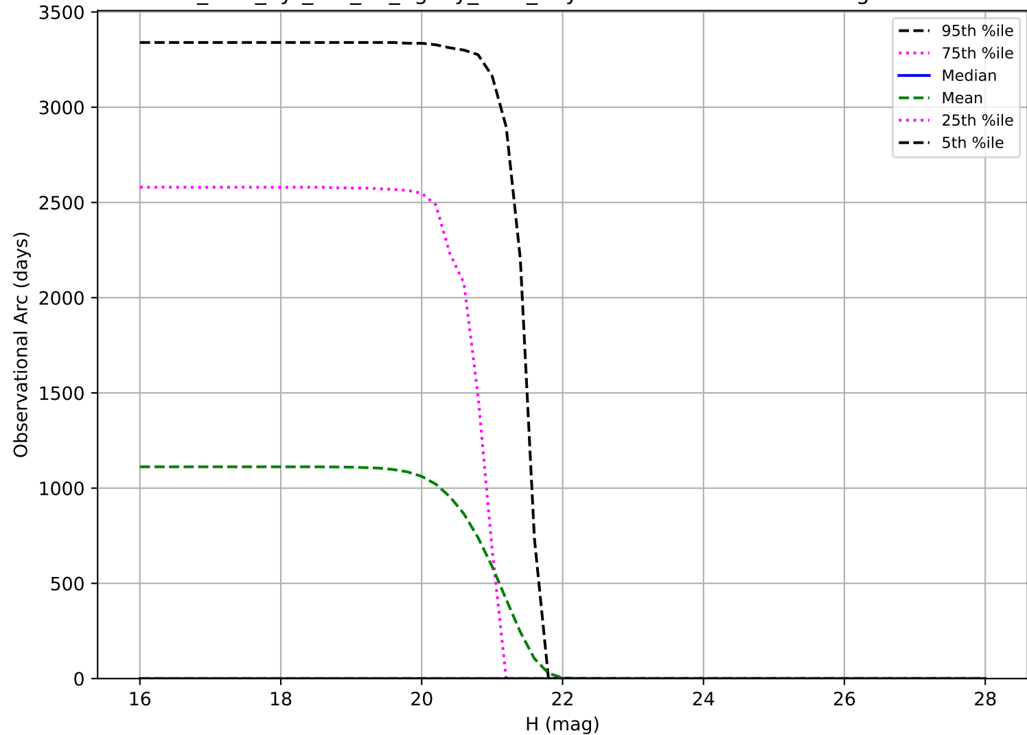
too_elab_2yr_r64_d2_ugrizy_v3.4_10yrs: Observational Arc Length Vatira
