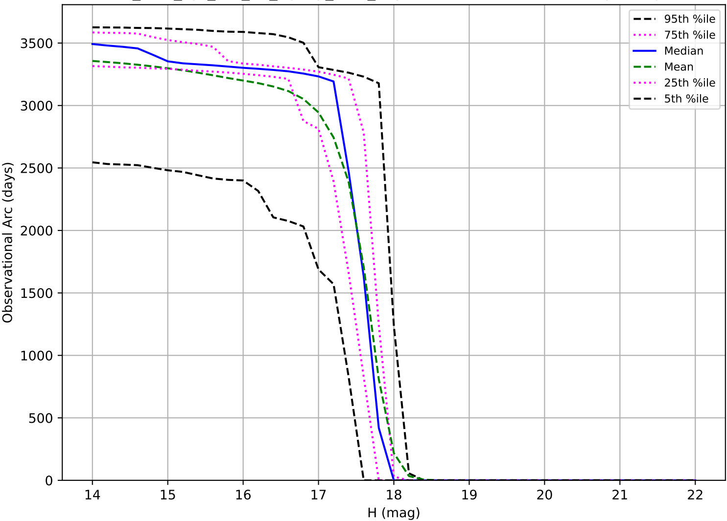
too_elab_2yr_r64_d2_ugrizy_v3.4_10yrs: Observational Arc Length Trojan
