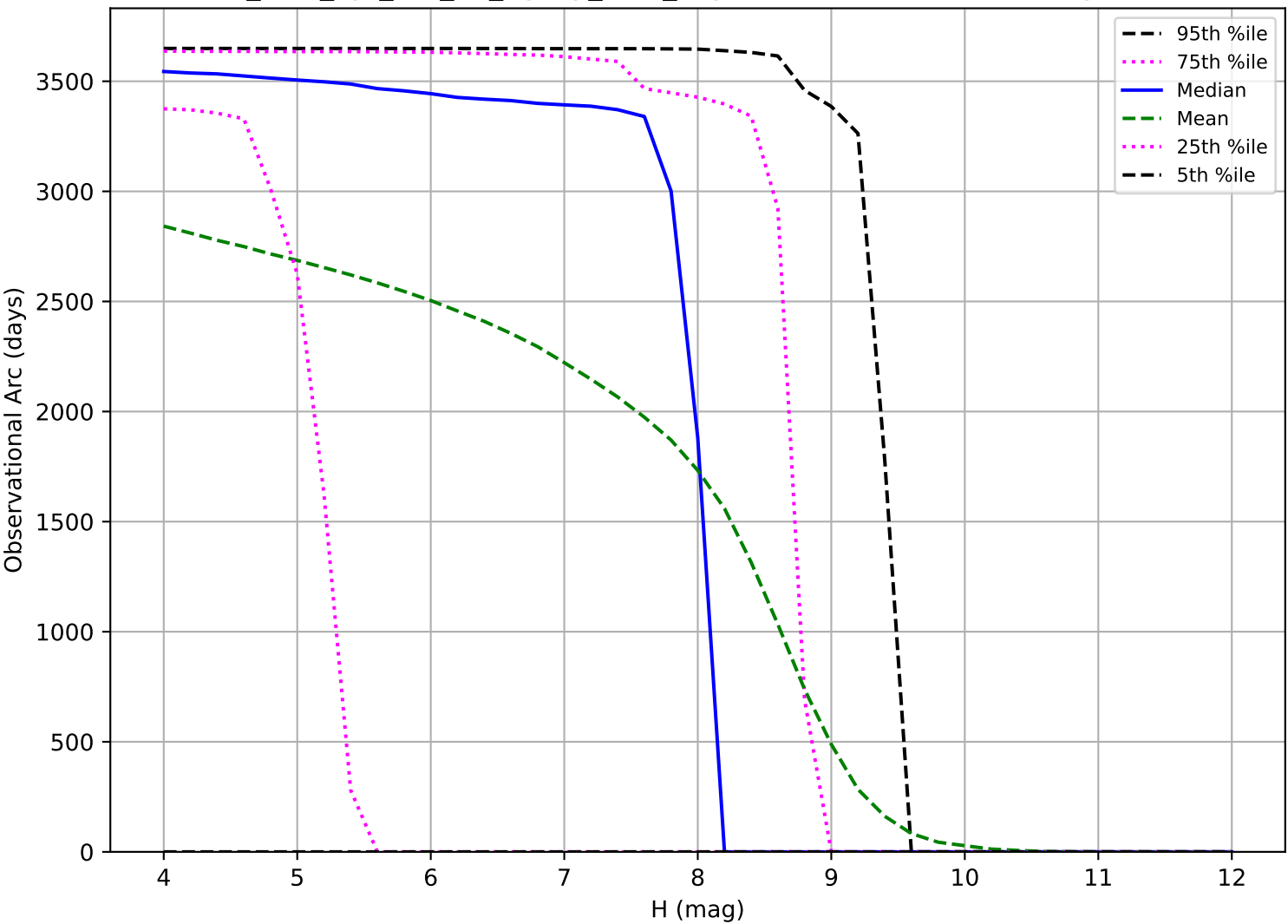
too_elab_2yr_r64_d2_ugrizy_v3.4_10yrs: Observational Arc Length TNO
