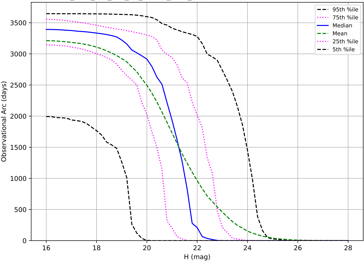
too_elab_2yr_r64_d2_ugrizy_v3.4_10yrs: Observational Arc Length PHA
