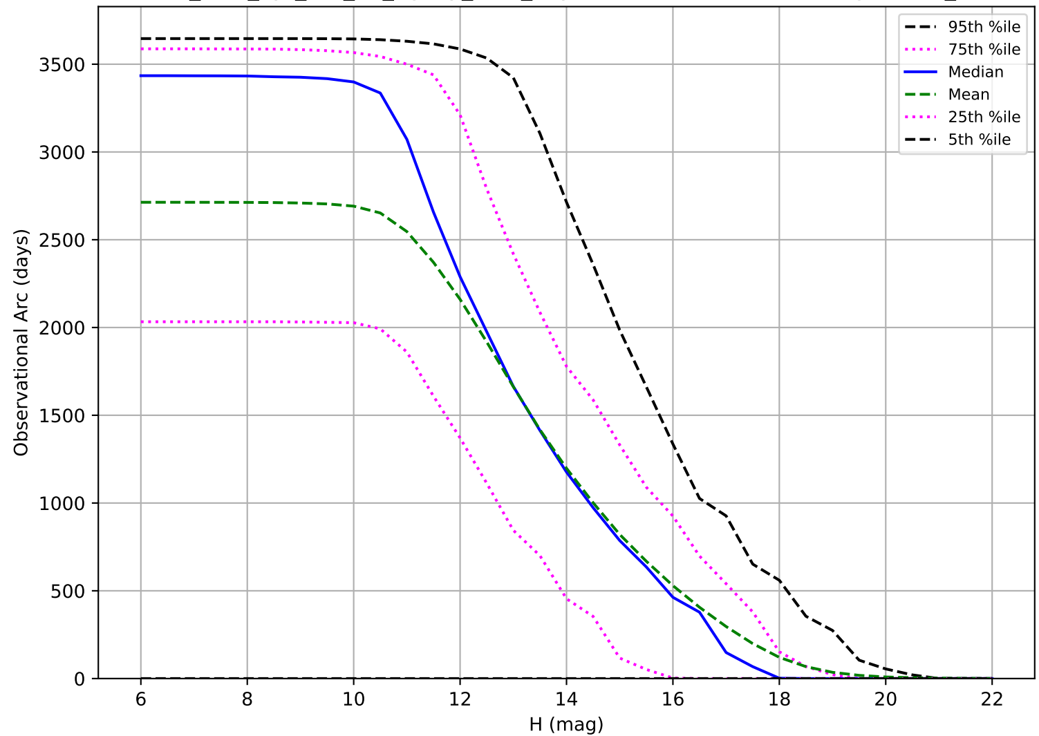
too_elab_2yr_r64_d2_ugrizy_v3.4_10yrs: Observational Arc Length OCC_r5
