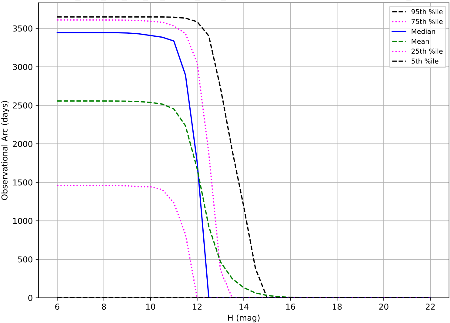
too_elab_2yr_r64_d2_ugrizy_v3.4_10yrs: Observational Arc Length OCC_r20
