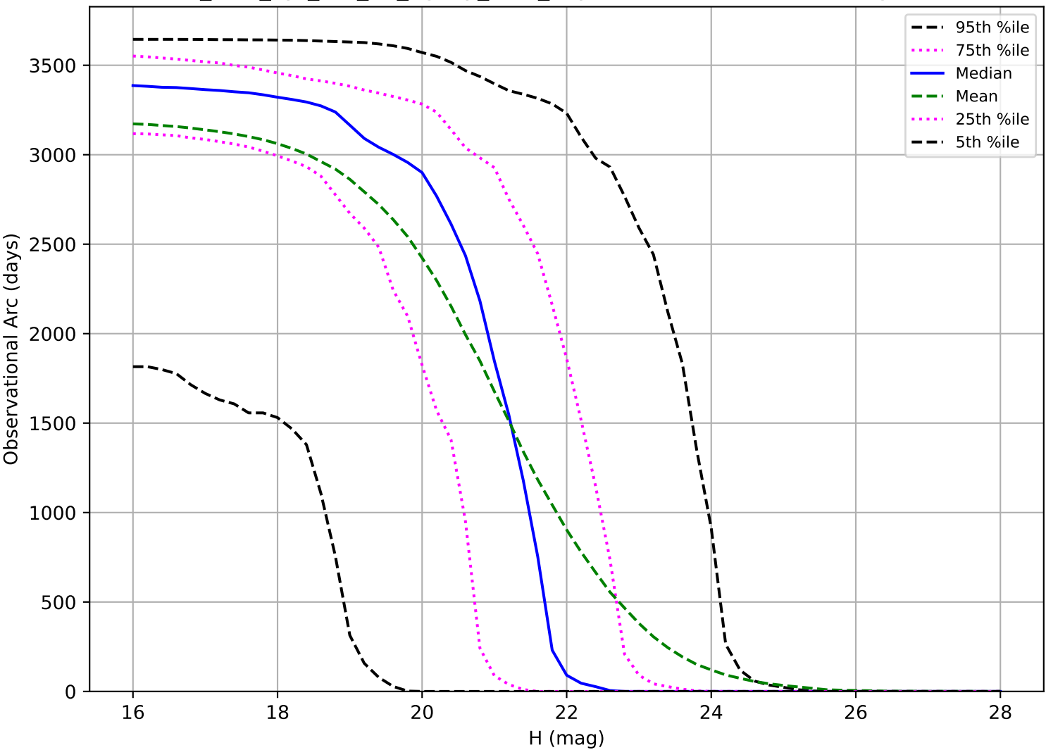
too_elab_2yr_r64_d2_ugrizy_v3.4_10yrs: Observational Arc Length NEO
