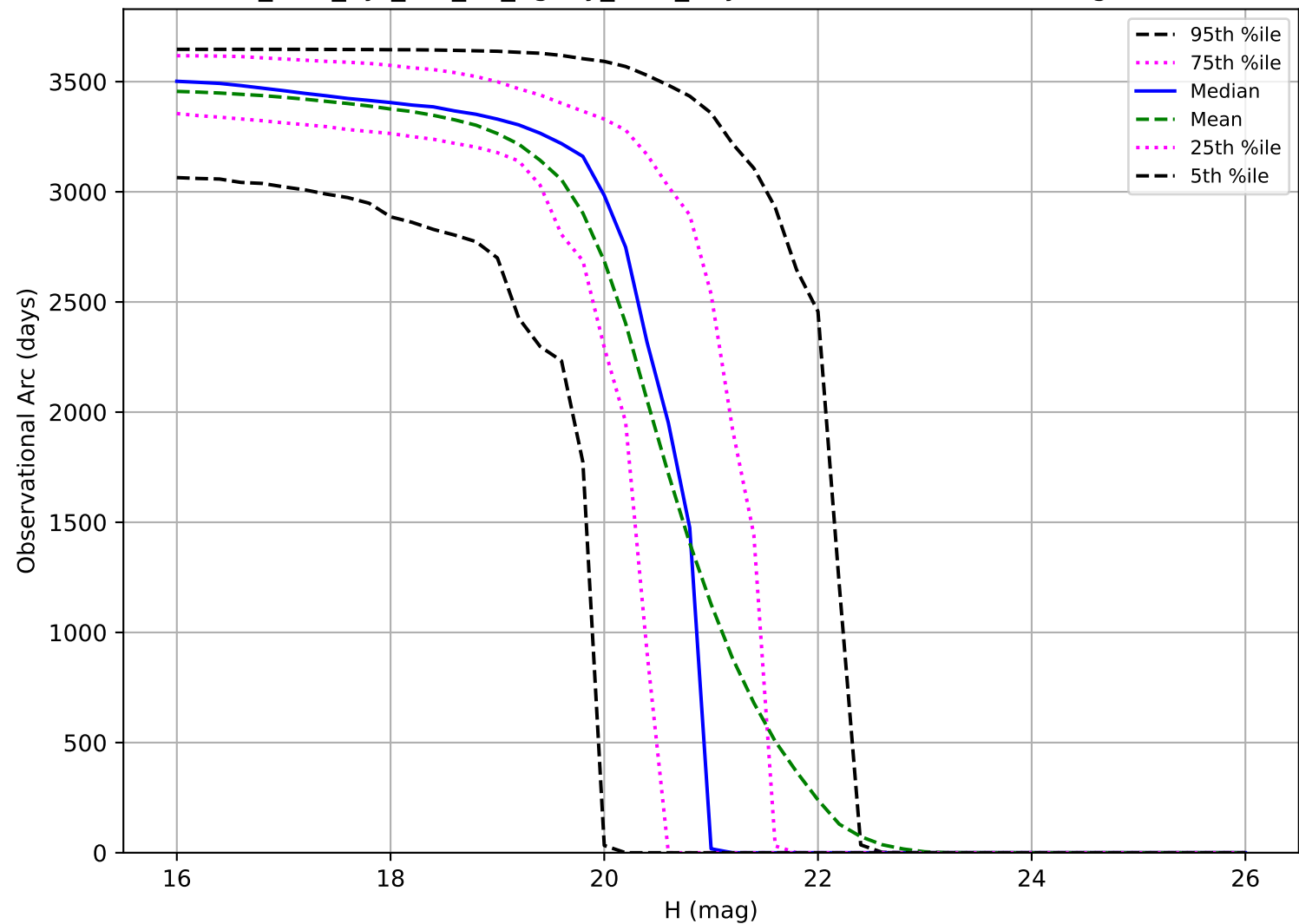
too_elab_2yr_r64_d2_ugrizy_v3.4_10yrs: Observational Arc Length MBA
