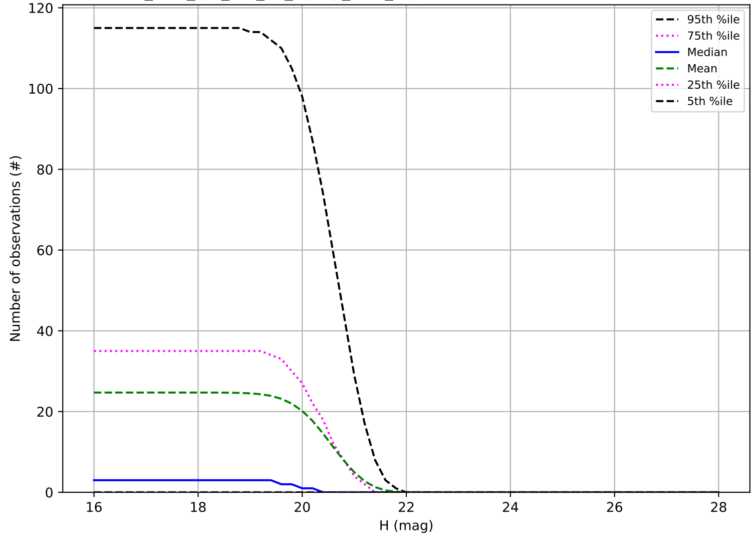
too_elab_2yr_r64_d2_ugrizy_v3.4_10yrs: Number of observations Vatira
