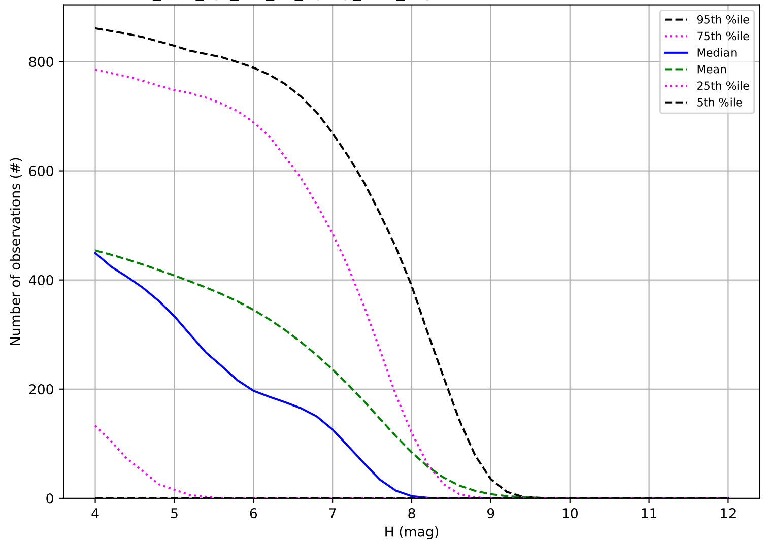
too_elab_2yr_r64_d2_ugrizy_v3.4_10yrs: Number of observations TNO
