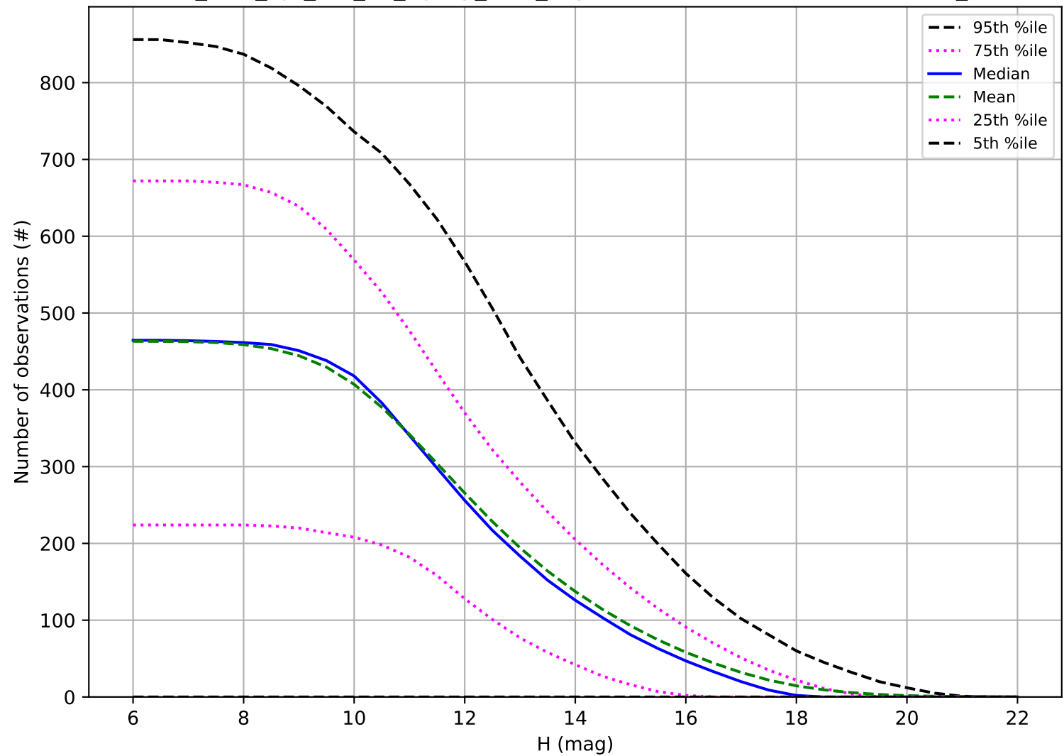
too_elab_2yr_r64_d2_ugrizy_v3.4_10yrs: Number of observations OCC_r5
