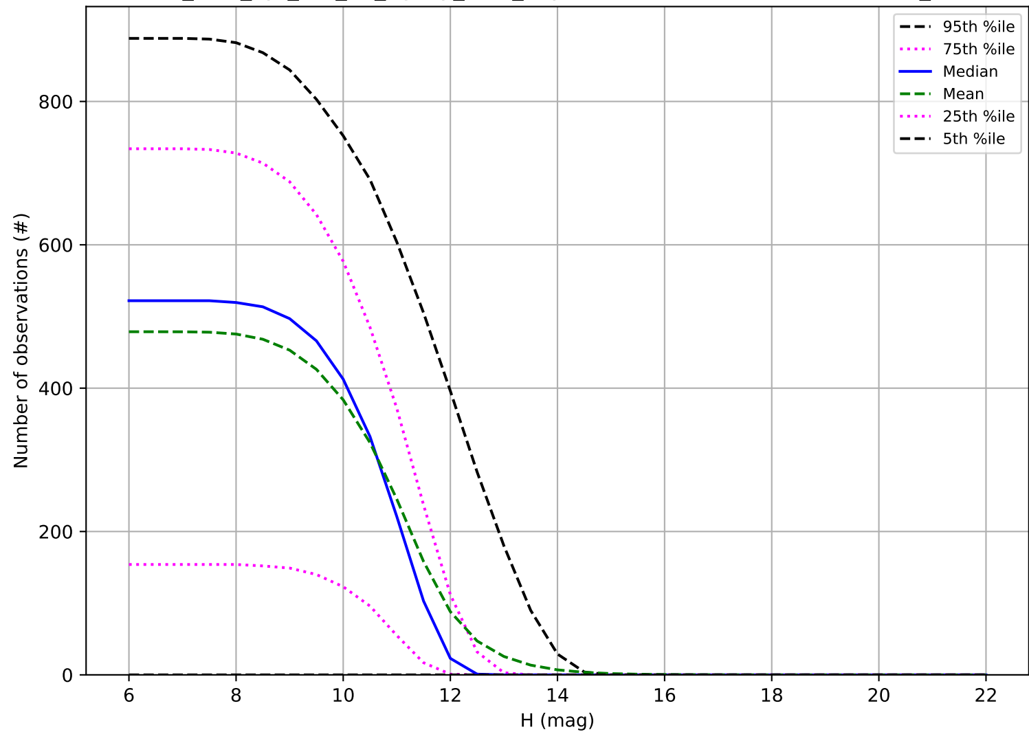
too_elab_2yr_r64_d2_ugrizy_v3.4_10yrs: Number of observations OCC_r20
