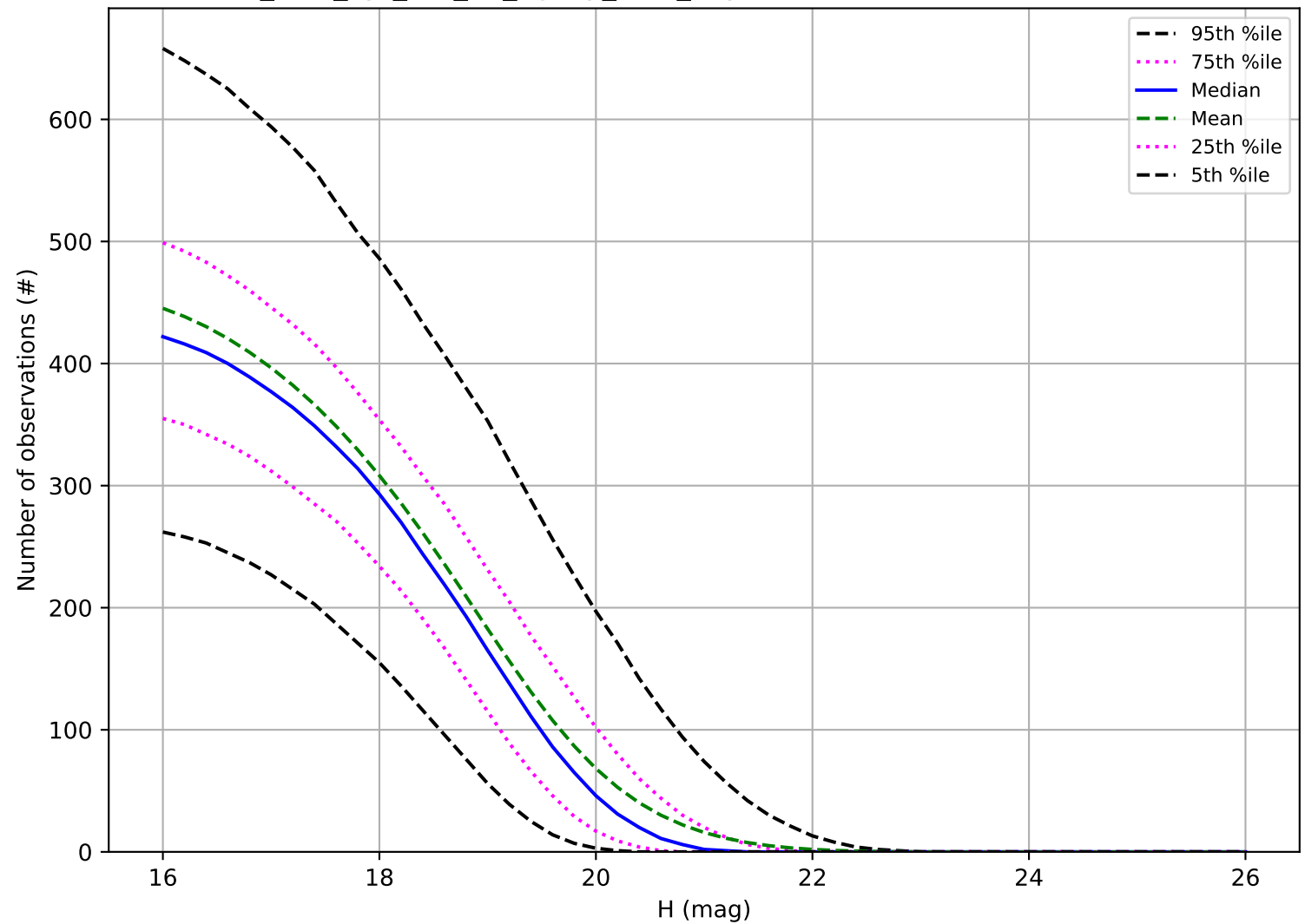
too_elab_2yr_r64_d2_ugrizy_v3.4_10yrs: Number of observations MBA
