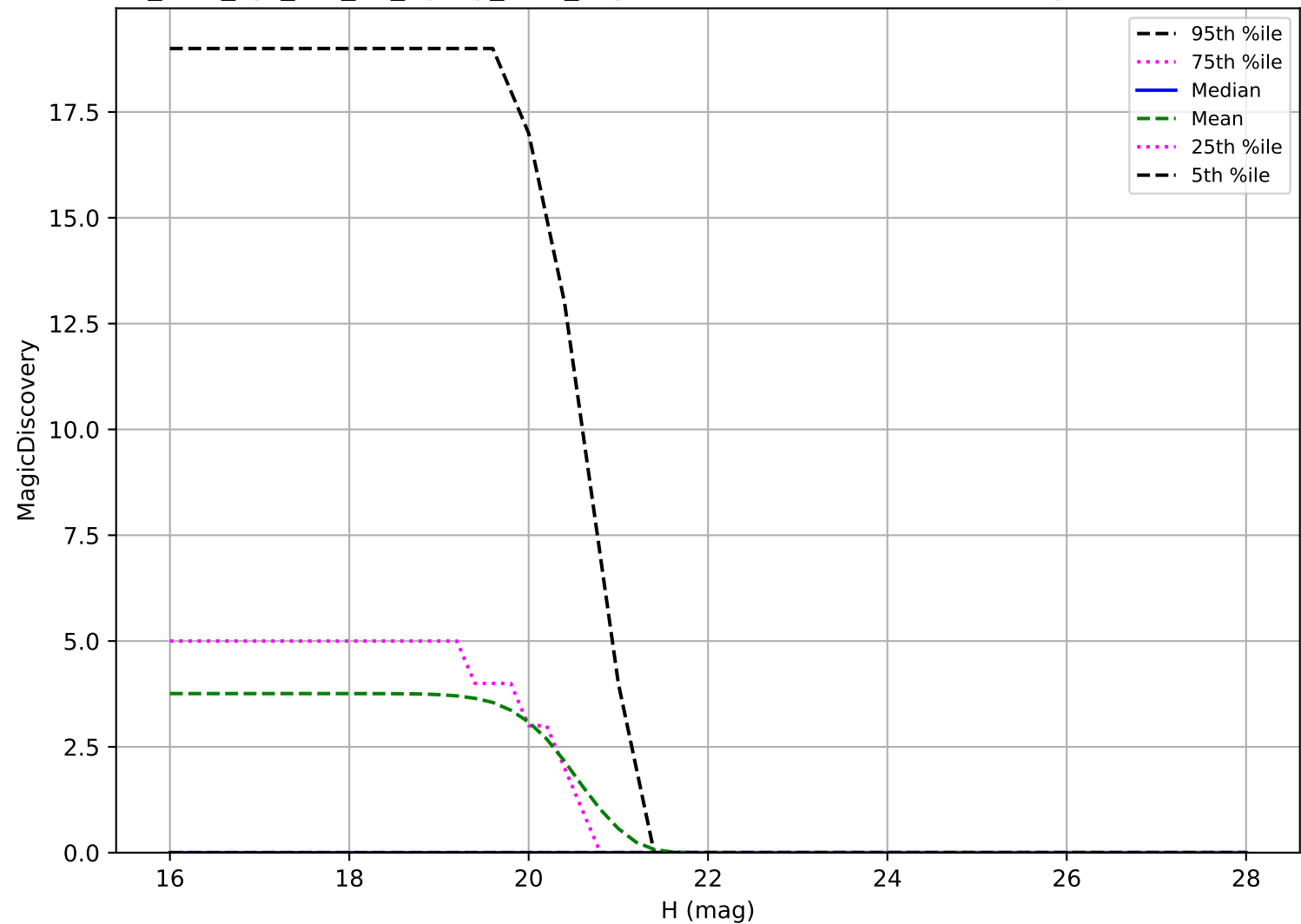
too_elab_2yr_r64_d2_ugrizy_v3.4_10yrs: Vatira 6 detections in 60 nights detection loss
