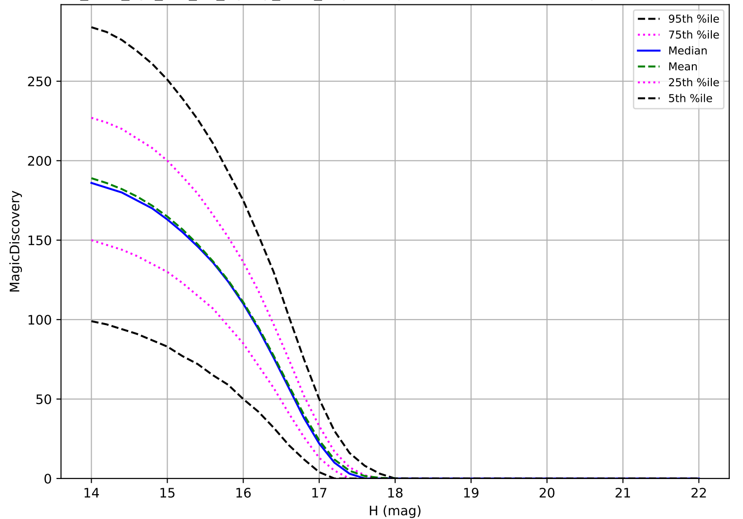
too_elab_2yr_r64_d2_ugrizy_v3.4_10yrs: Trojan 6 detections in 60 nights detection loss
