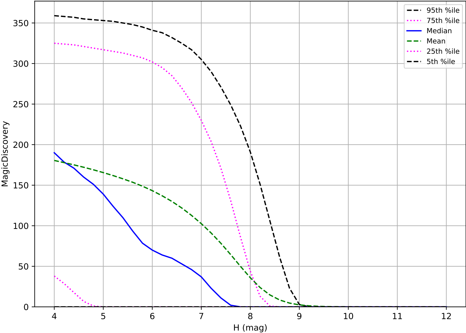
too_elab_2yr_r64_d2_ugrizy_v3.4_10yrs: TNO 6 detections in 60 nights detection loss
