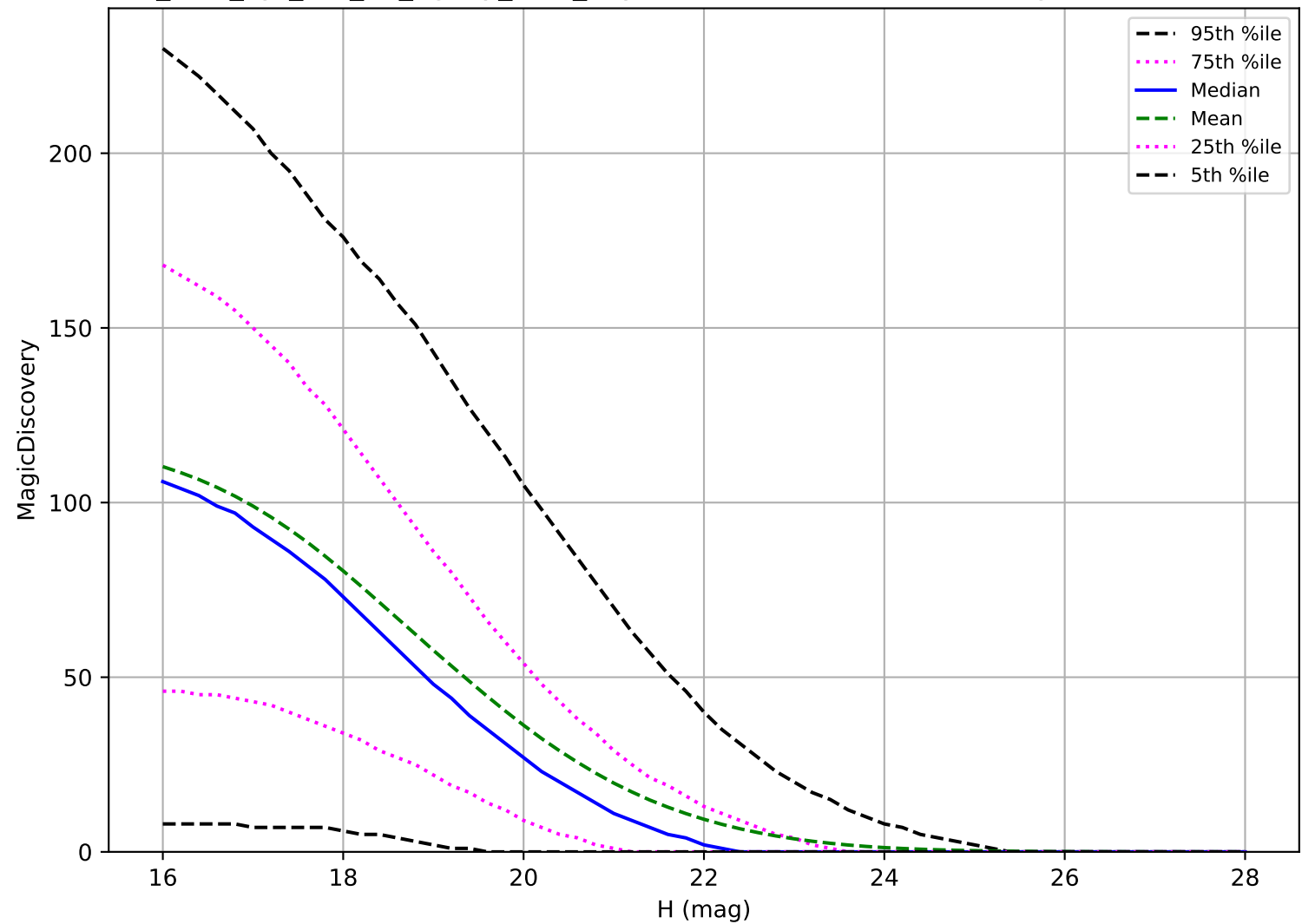
too_elab_2yr_r64_d2_ugrizy_v3.4_10yrs: PHA 6 detections in 60 nights detection loss
