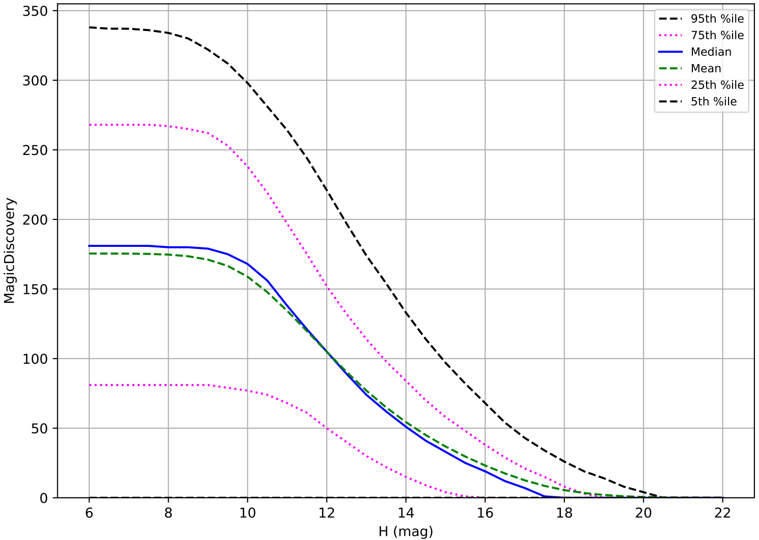
too_elab_2yr_r64_d2_ugrizy_v3.4_10yrs: OCC_r5 6 detections in 60 nights detection loss
