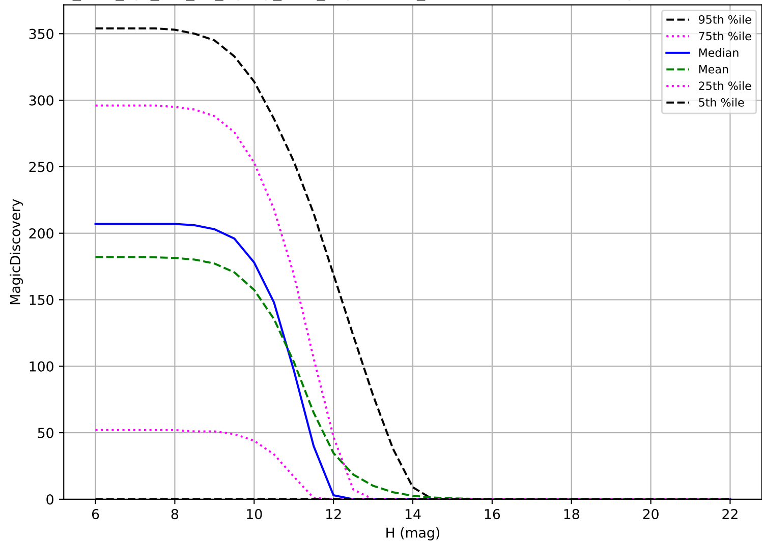
too_elab_2yr_r64_d2_ugrizy_v3.4_10yrs: OCC_r20 6 detections in 60 nights detection loss
