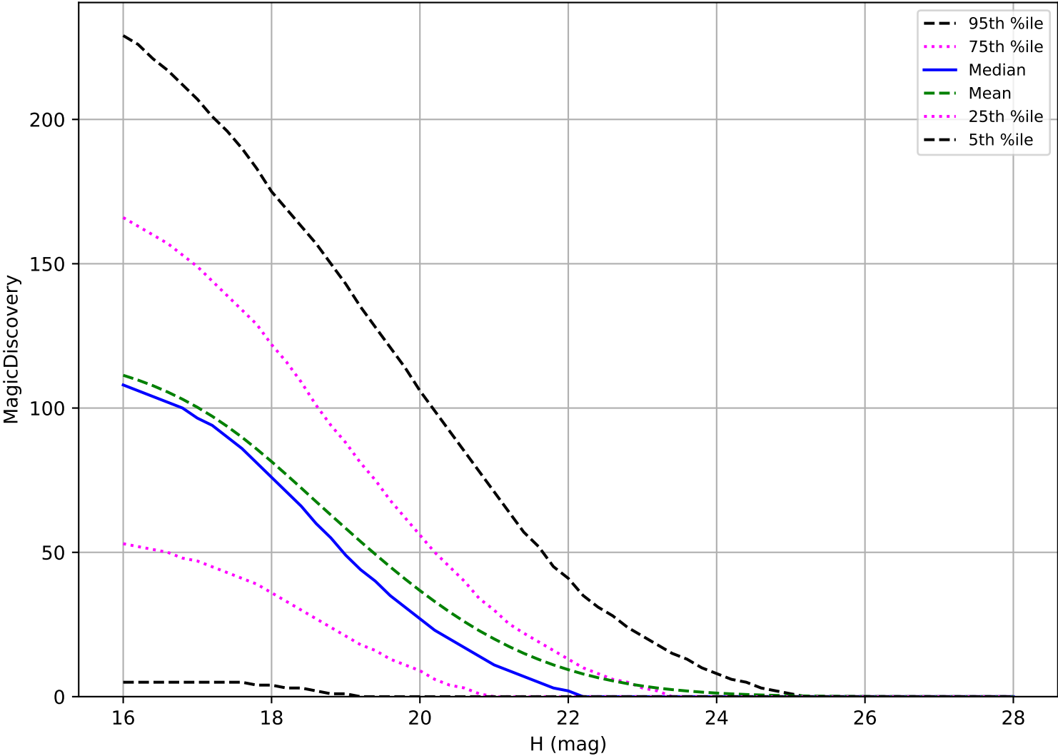
too_elab_2yr_r64_d2_ugrizy_v3.4_10yrs: NEO 6 detections in 60 nights detection loss
