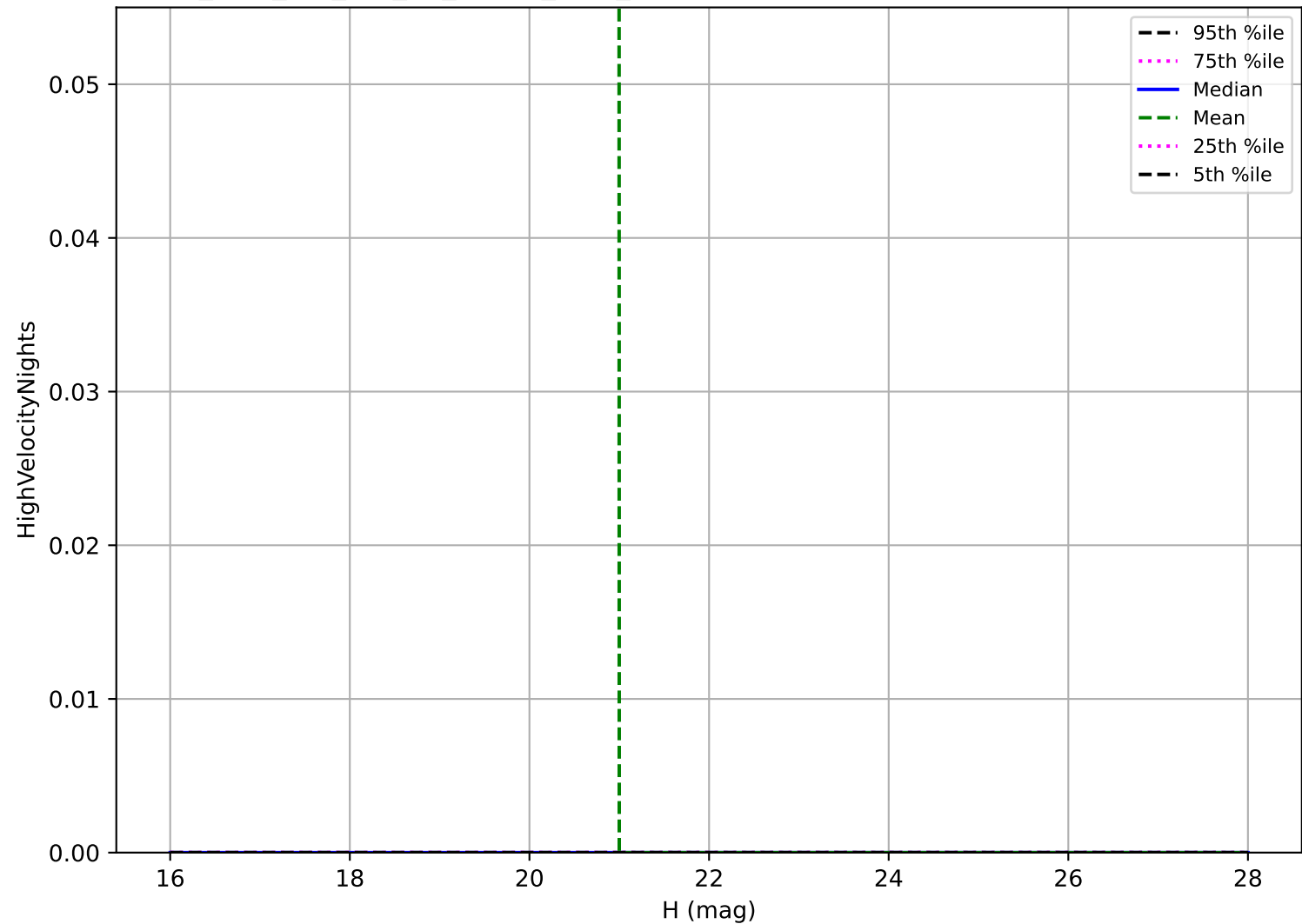
too_elab_2yr_r64_d2_ugrizy_v3.4_10yrs: Vatira High velocity pair detection loss
