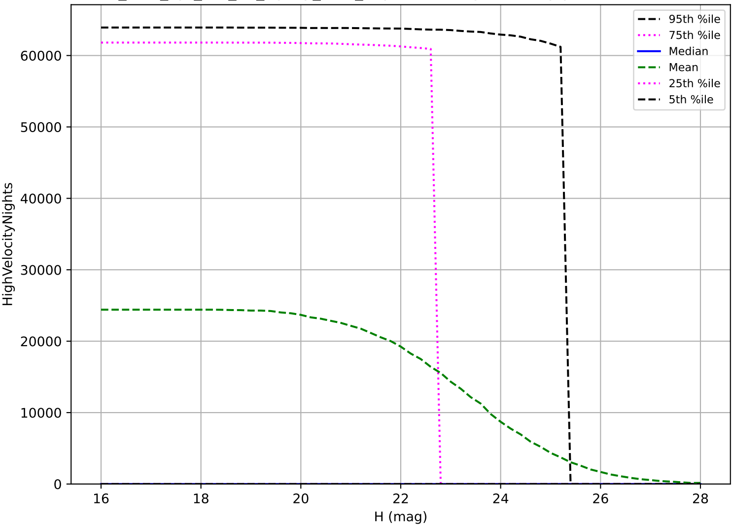
too_elab_2yr_r64_d2_ugrizy_v3.4_10yrs: PHA High velocity pair detection loss
