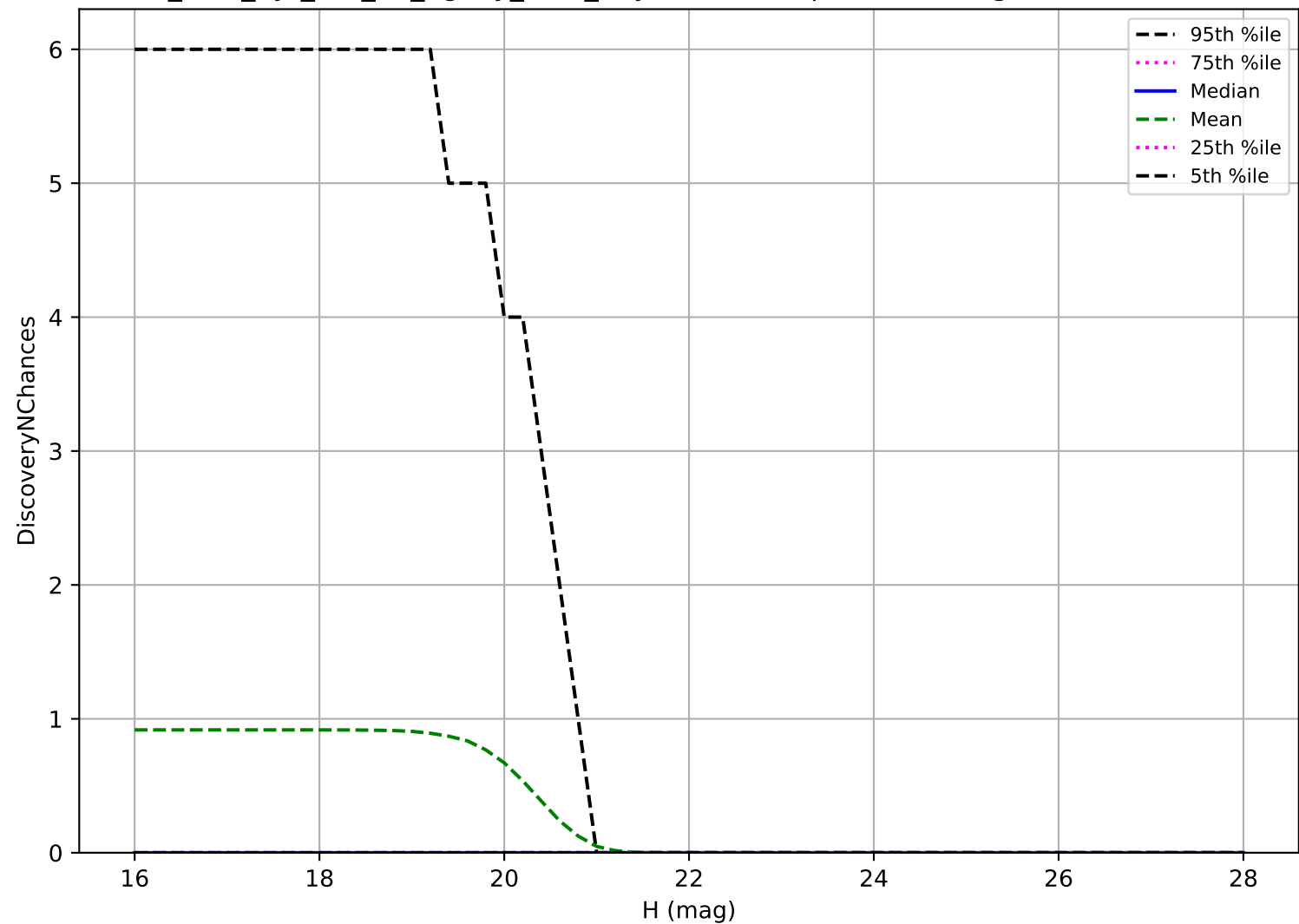
too_elab_2yr_r64_d2_ugrizy_v3.4_10yrs: Vatira 3 pairs in 15 nights detection loss
