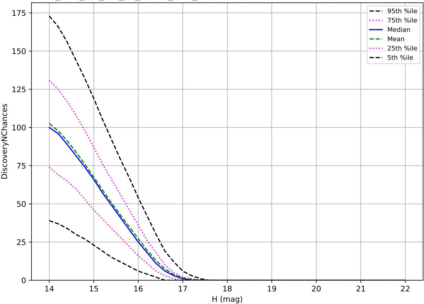
too_elab_2yr_r64_d2_ugrizy_v3.4_10yrs: Trojan 3 pairs in 15 nights detection loss
