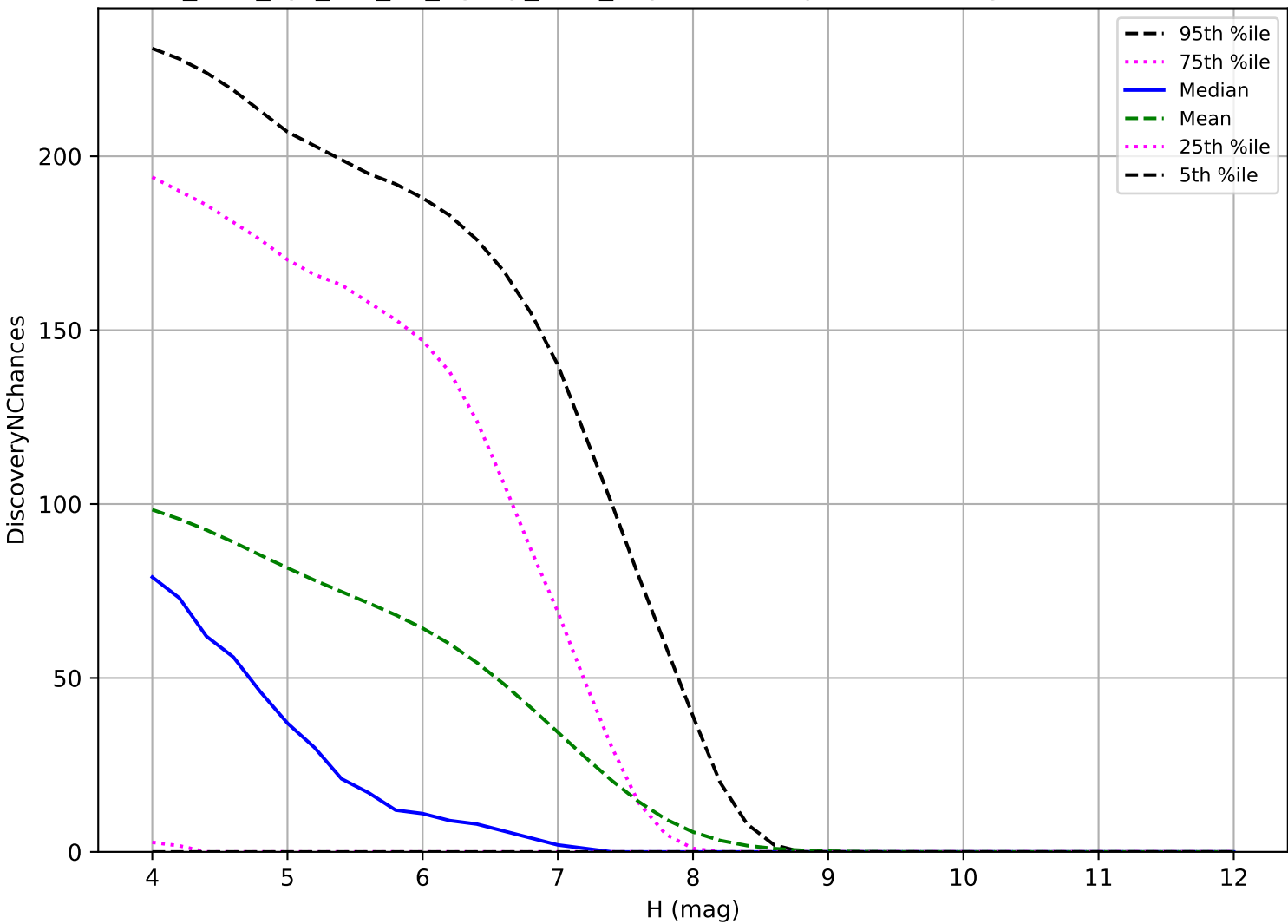
too_elab_2yr_r64_d2_ugrizy_v3.4_10yrs: TNO 3 pairs in 15 nights detection loss
