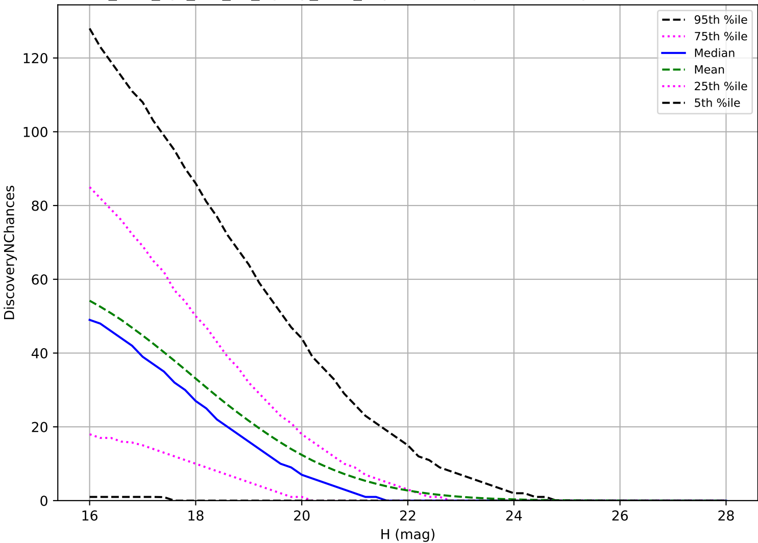
too_elab_2yr_r64_d2_ugrizy_v3.4_10yrs: PHA 3 pairs in 15 nights detection loss
