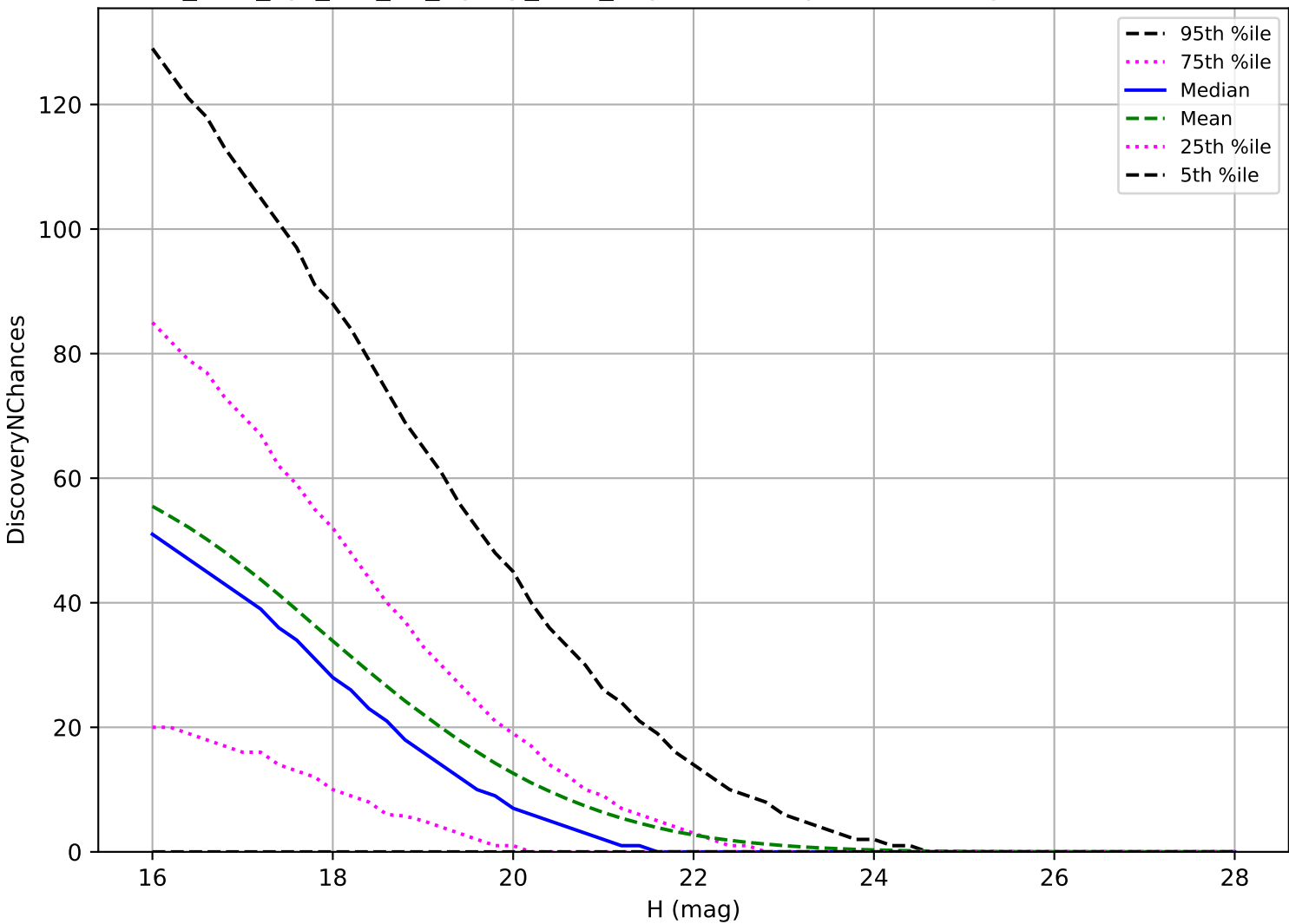
too_elab_2yr_r64_d2_ugrizy_v3.4_10yrs: NEO 3 pairs in 15 nights detection loss
