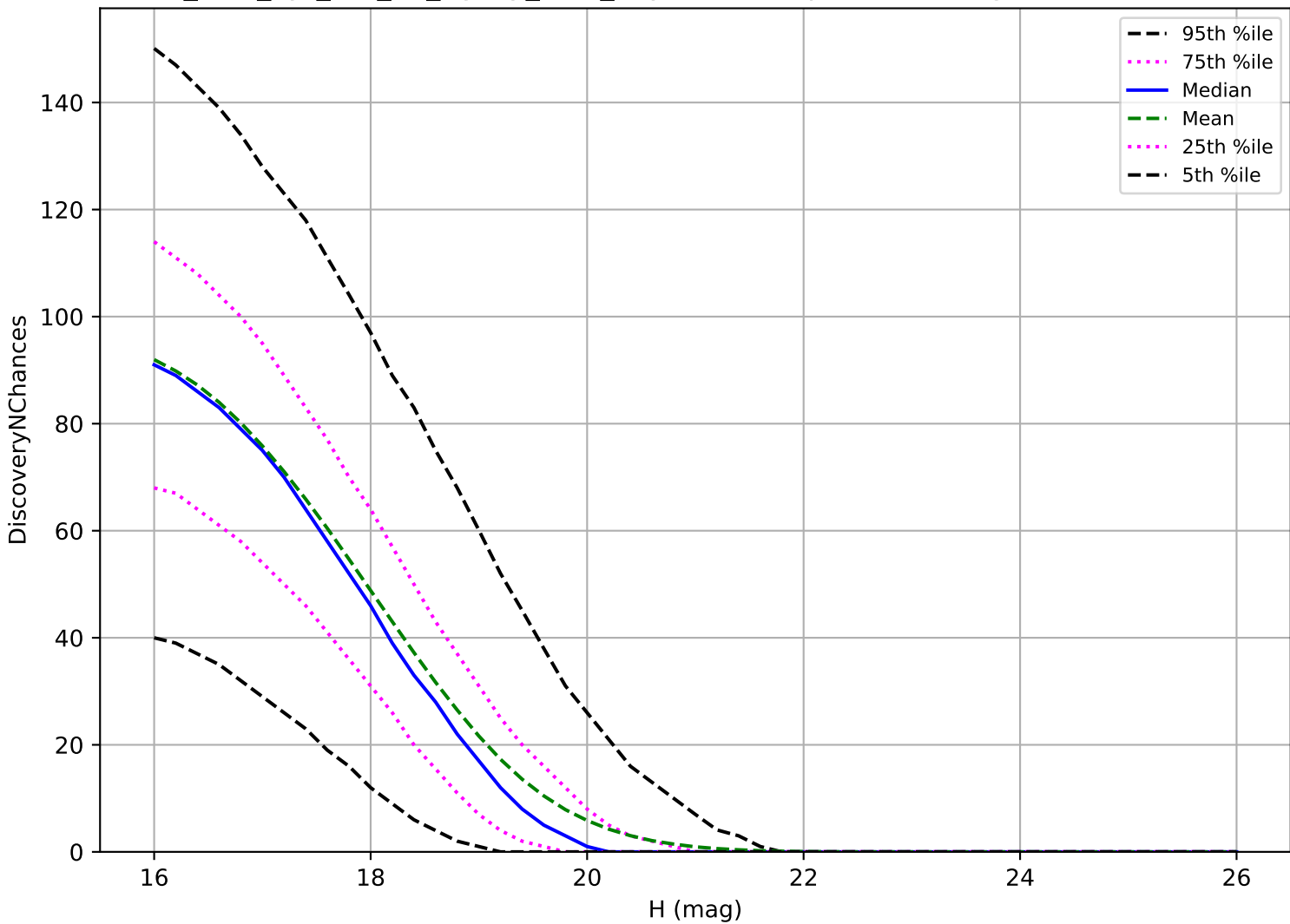
too_elab_2yr_r64_d2_ugrizy_v3.4_10yrs: MBA 3 pairs in 15 nights detection loss
