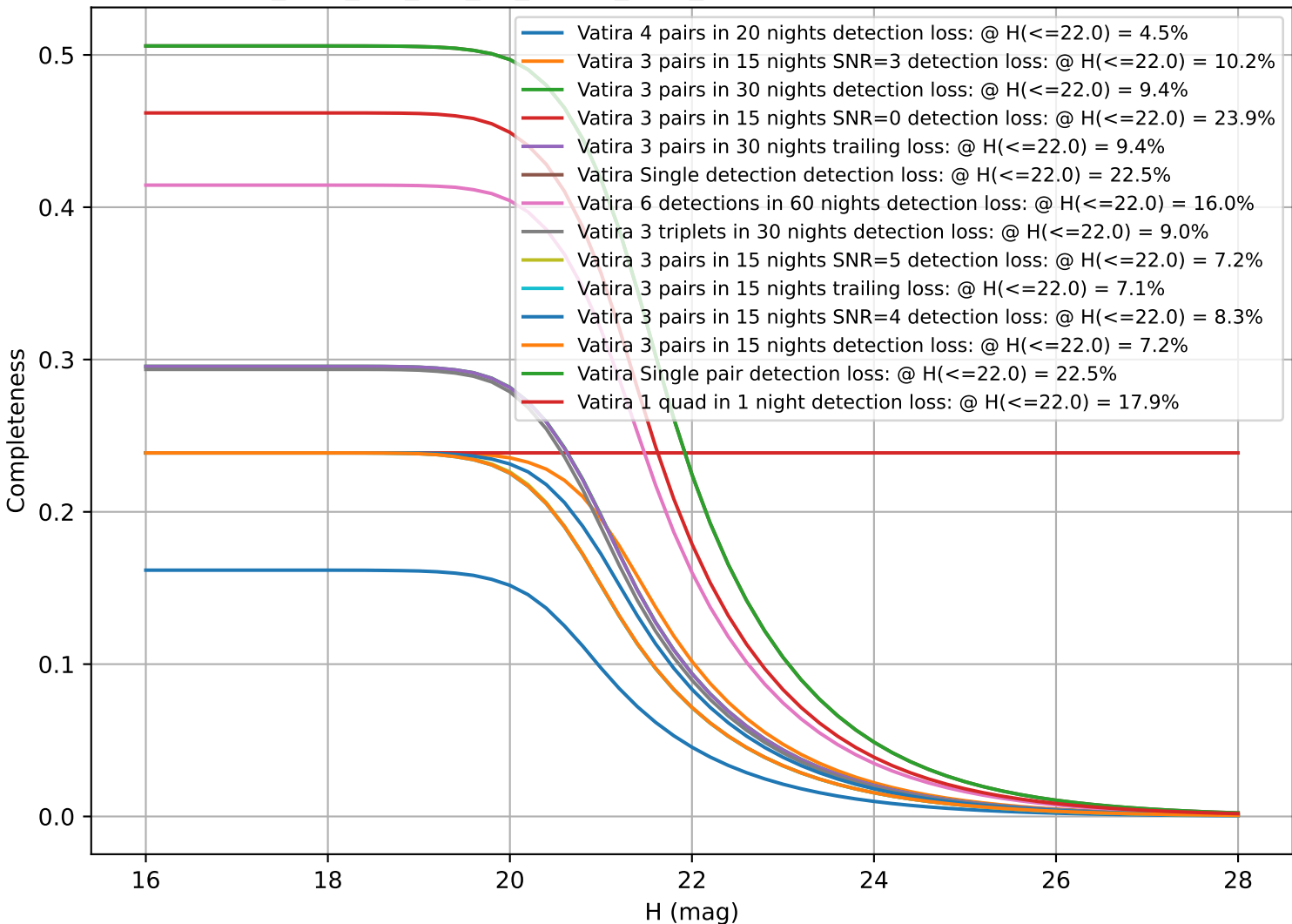
too_elab_2yr_r64_d2_ugrizy_v3.4_10yrs: CumulativeCompleteness
