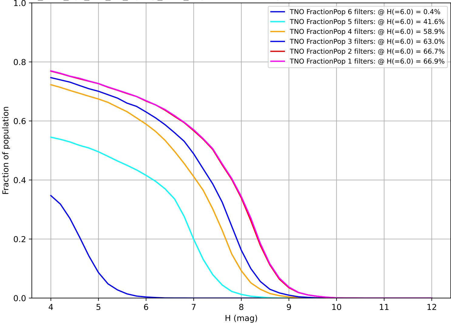
too_elab_2yr_r64_d2_ugrizy_v3.4_10yrs: Fraction of population with colors in X filters TNO
