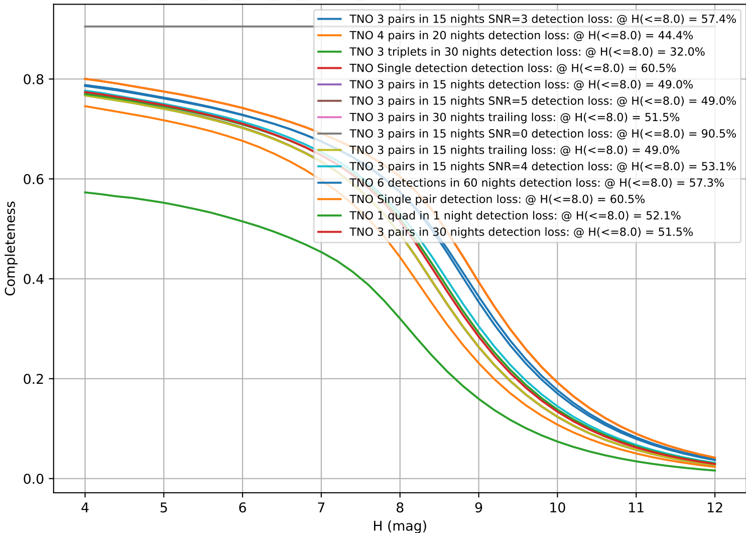
too_elab_2yr_r64_d2_ugrizy_v3.4_10yrs: CumulativeCompleteness
