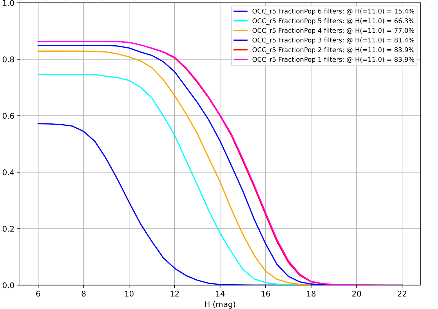
too_elab_2yr_r64_d2_ugrizy_v3.4_10yrs: Fraction of population with colors in X filters OCC_r5
