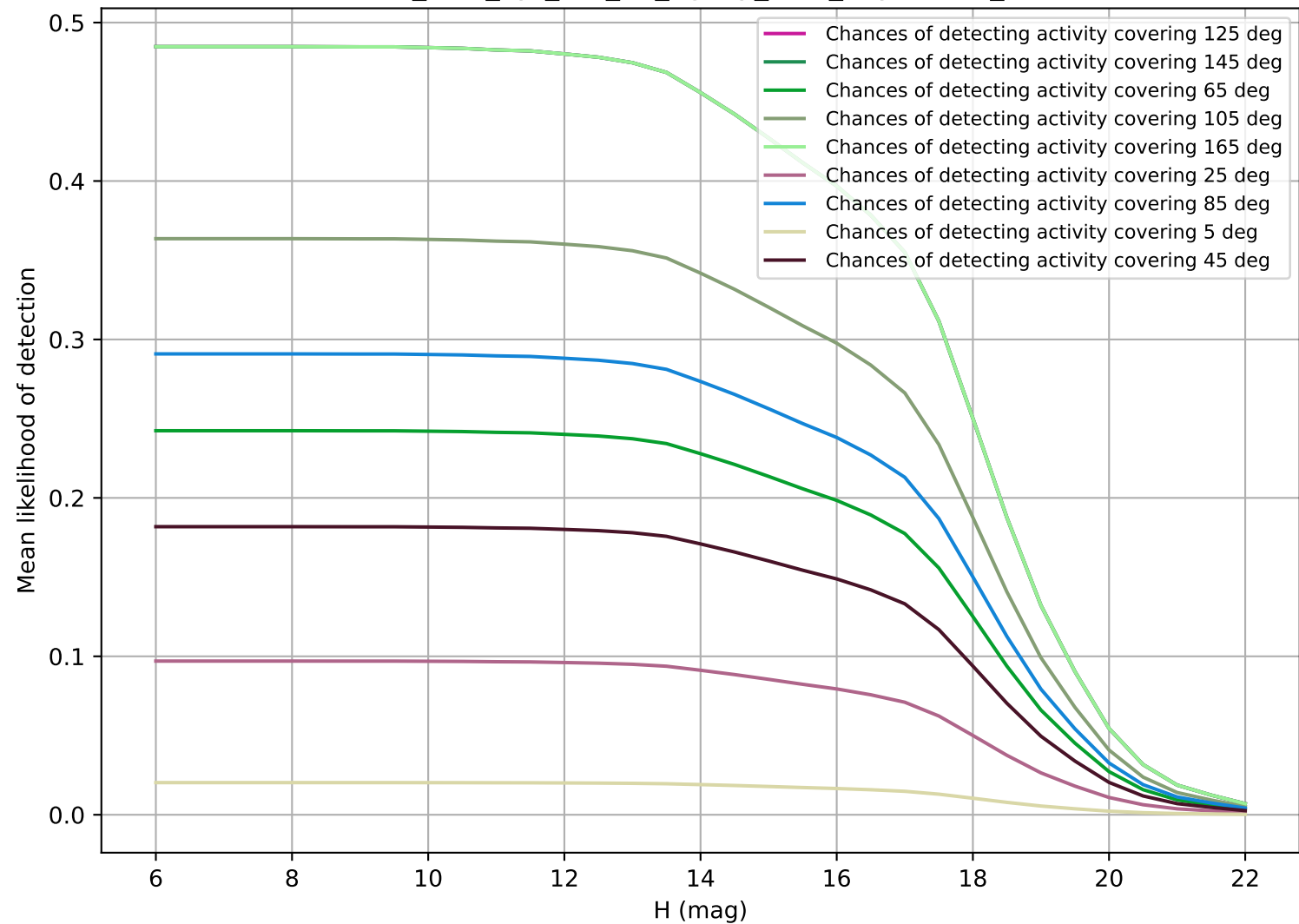
too_elab_2yr_r64_d2_ugrizy_v3.4_10yrs OCC_r5
